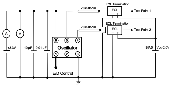
Fig.1 Test Circuit
