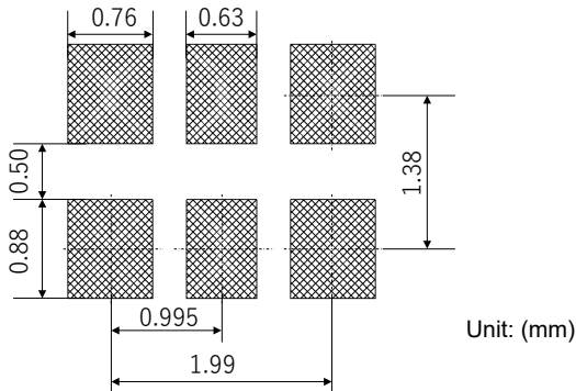
Fig.4 Land pattern
