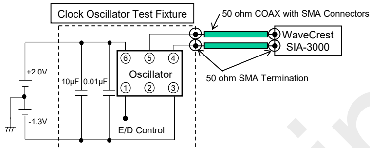
Fig.3 Jitter Test Circuit
