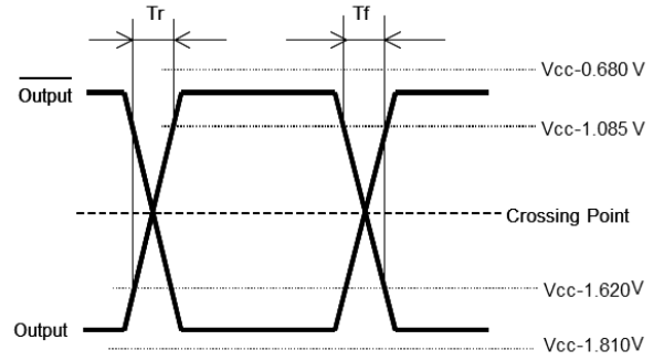
Fig.2 Clock Timing Chart
